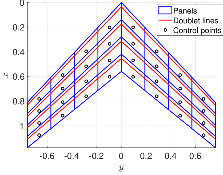
Figure 1: Panel grid used by the DLM
