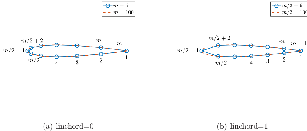
Figure 2: Chordwise panel numbering and distributions for the SDPM
