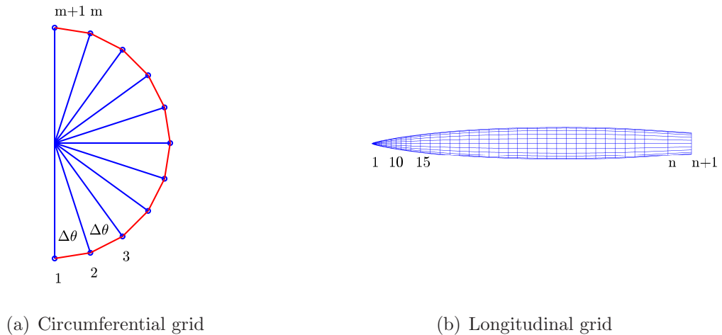
Figure 5: Circumferential and longitudinal discretization for fuselage used in SDPMflut
