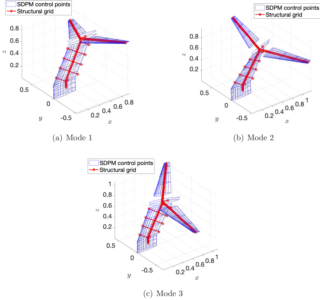
Figure 8: T-tail deformed parallel to the first three mode shapes[3].
