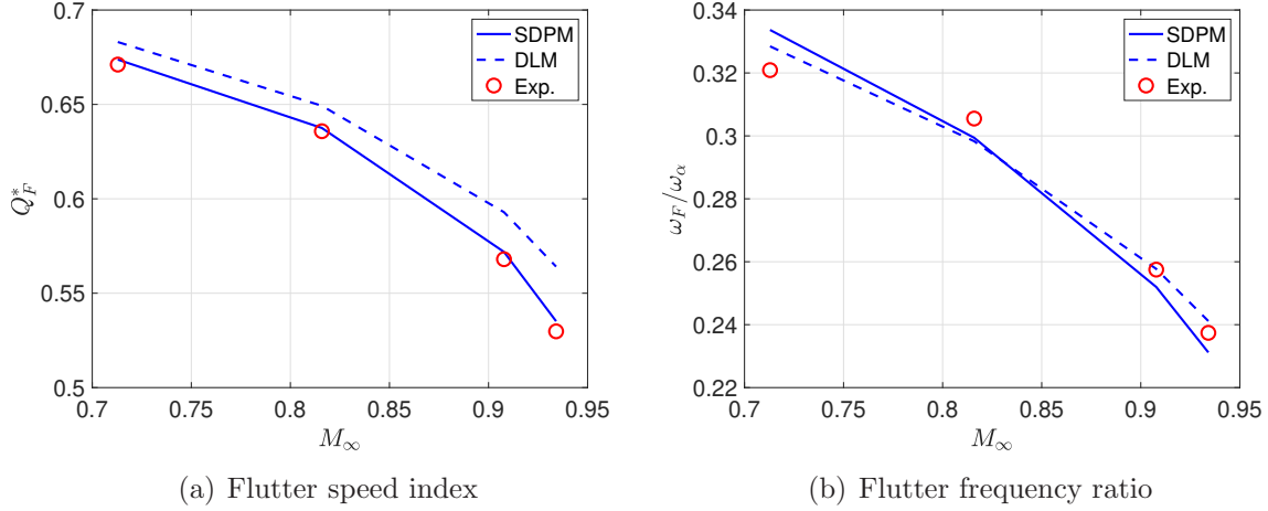
Figure 13: Variation of flutter speed index and flutter frequency ratio with Mach number for the NASATMX72799 test case with heavy winglets
