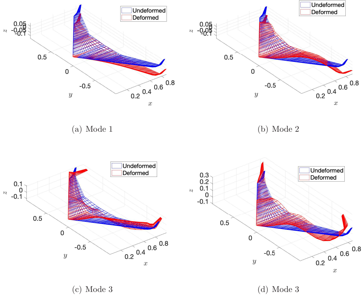
Figure 7: First four mode shapes of the NASA TMX 72799 wing with heavy winglet.
