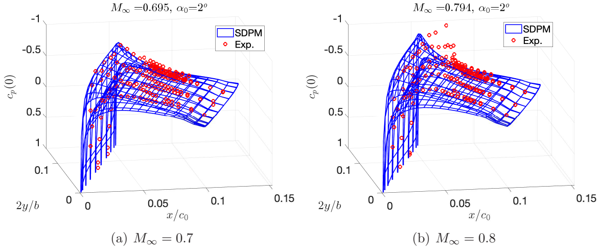
Figure 9: Steady pressure distributions for the NASATM8436 test case at two Mach numbers
