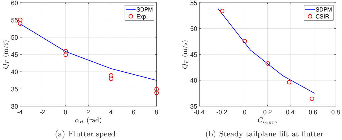
Figure 15: Variation of flutter speed with tailplane incidence and steady tailplane lift at flutter for the Van Zyl T-tail test case
