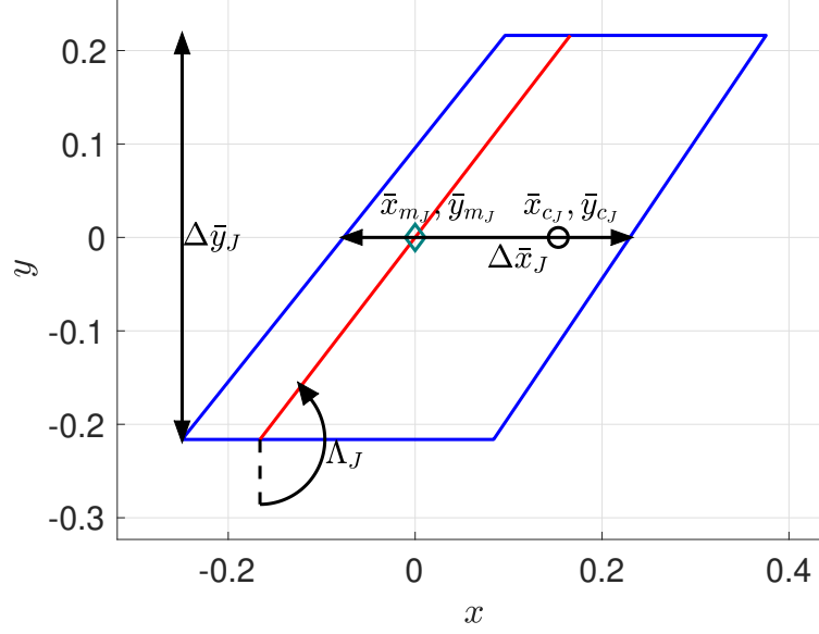
Figure 19: 2D view of J th panel in its own coordinate system
