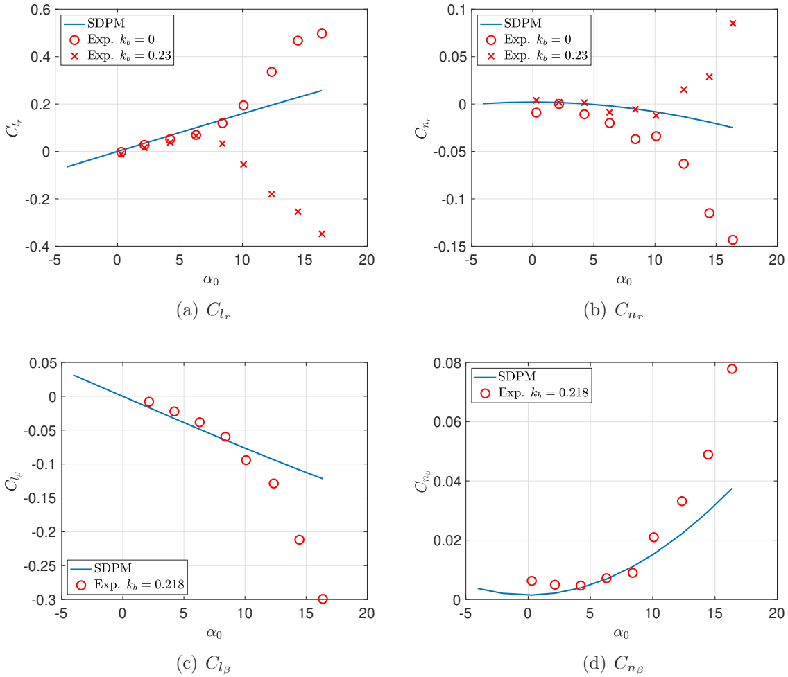
Figure 12: Variation of aerodynamic stability derivatives with steady pitch angle for the straight wing
