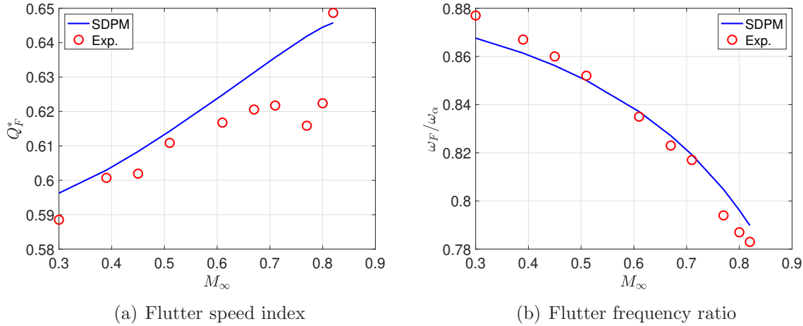
Figure 16: Variation of flutter speed index and flutter frequency ratio with Mach number for the NACA0012 test case
