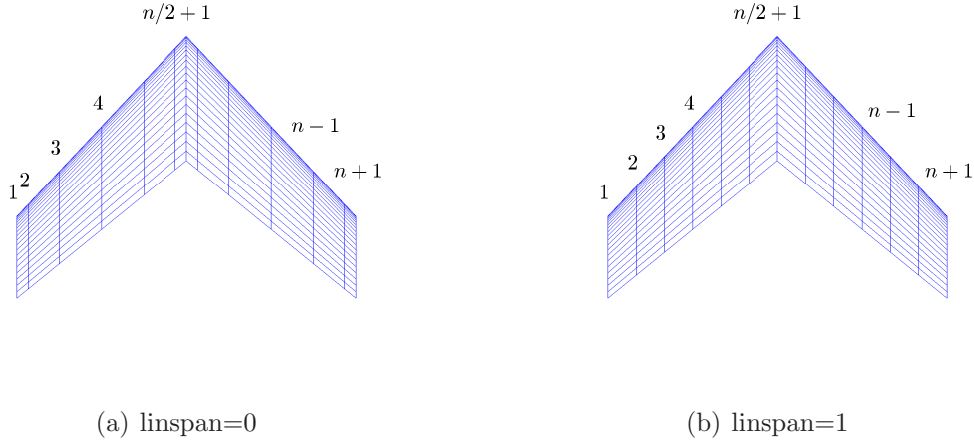
Figure 3: Spanwise panel numbering and distributions for the SDPM
