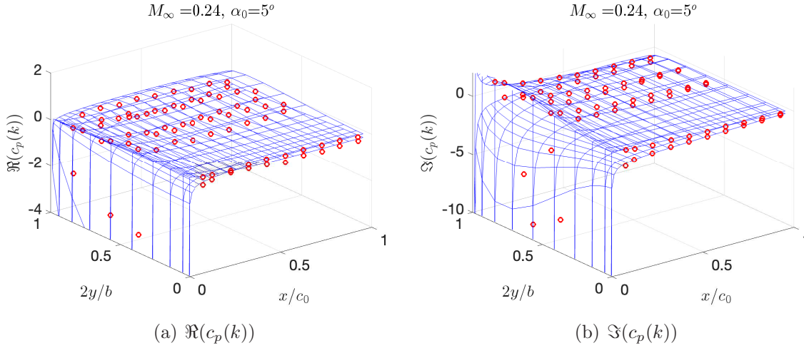
Figure 10: Real and imaginary parts of the pressure distribution for the NASATND344 test case at M_\infty = 24 , \alpha_0 = 5^\circ
